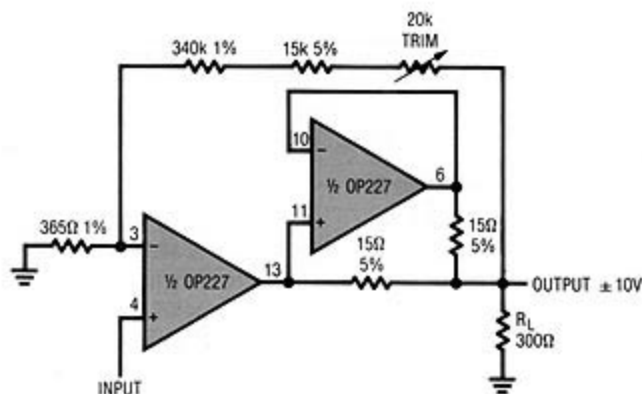
Precision Amplifier Drives 300\Omega Load to \pm 10\text{V} with 0.05% Accuracy
