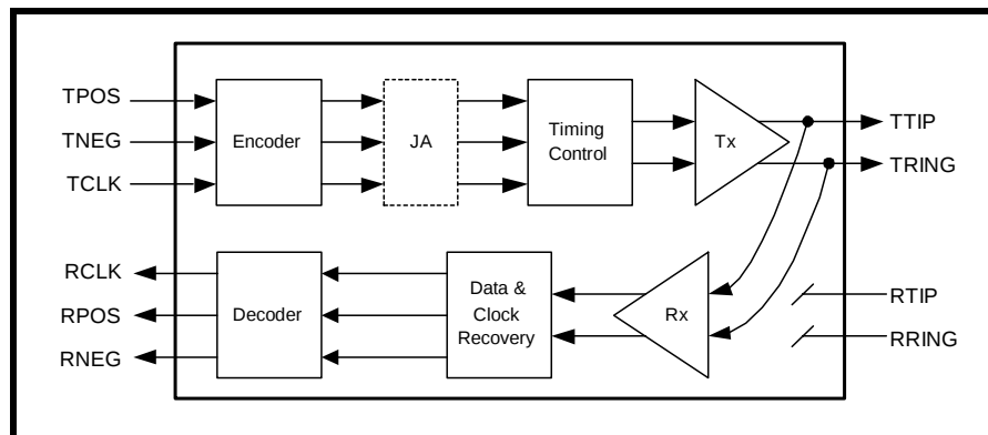
FIGURE 20. LOCAL ANALOG LOOP-BACK SIGNAL FLOW
