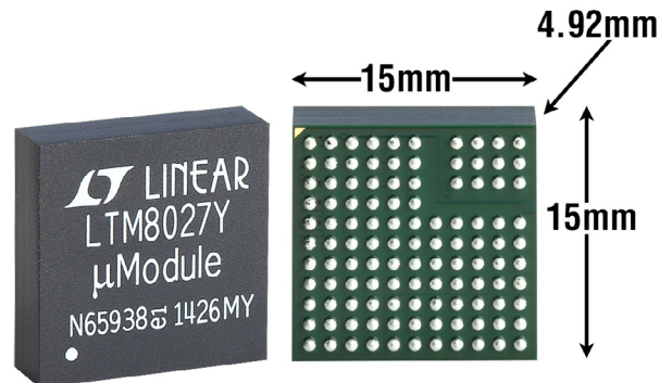
BGA
