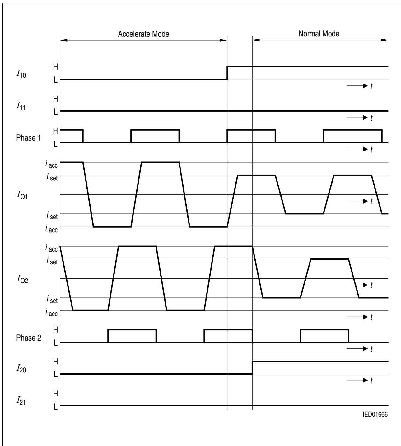
Figure 7 Full-Step Operation
