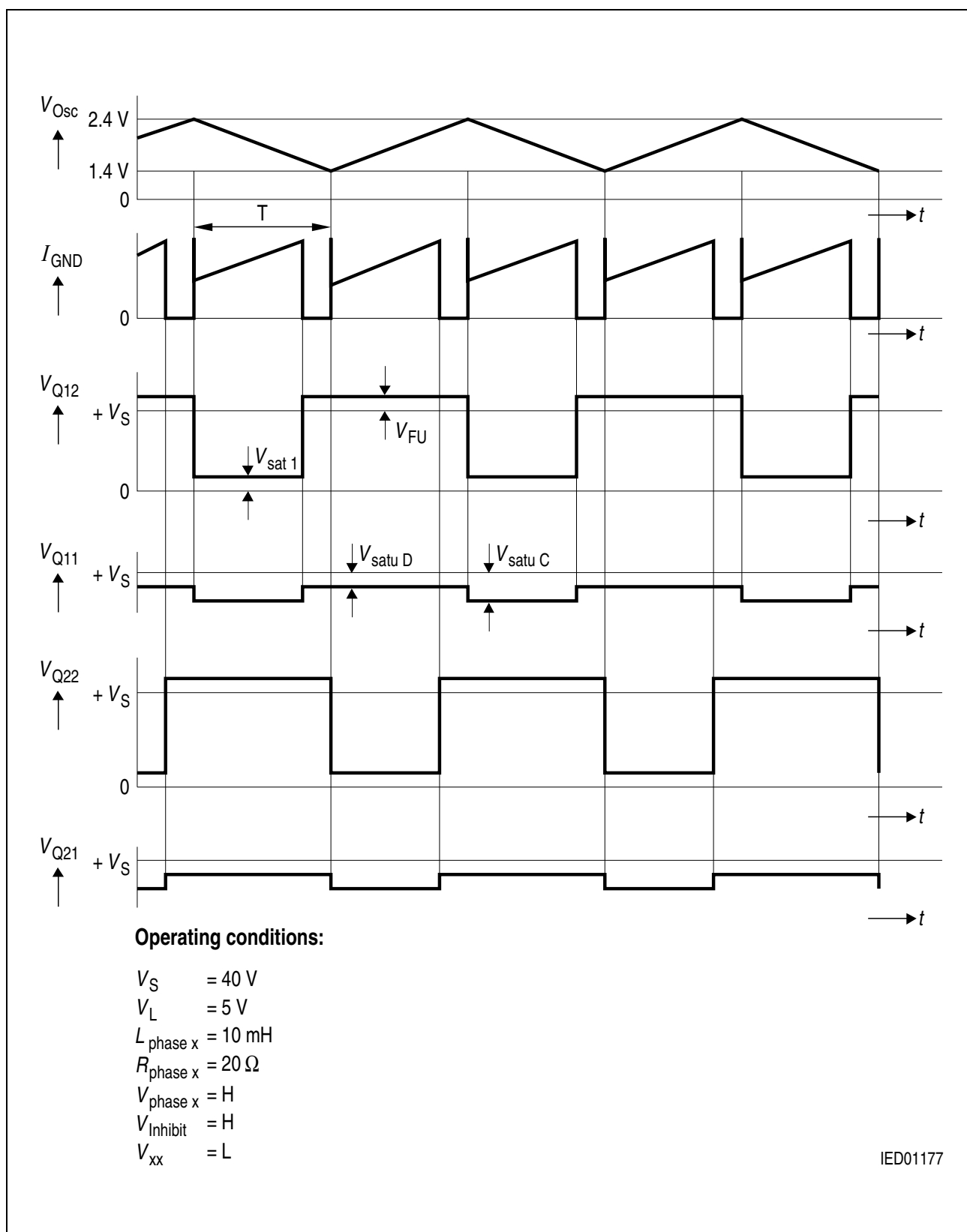
Figure 11 Current Control
