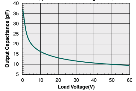
Output Capacitance vs. Load Voltage ( I_F=1mA, f=1MHz, T_A=25^{\circ}C )
