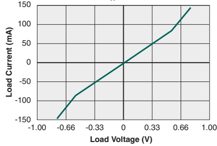
Typical Load Current vs. Load Voltage ( T_A=25^{\circ}C )
