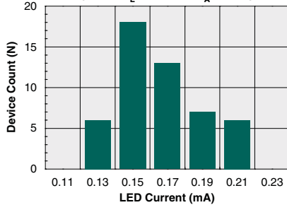
Typical I F for Switch Operation (N=50, I L =150mA, T A =25°C)
