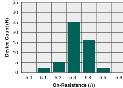
Typical On-Resistance Distribution (N=50, I L =150mA, T A =25°C)
