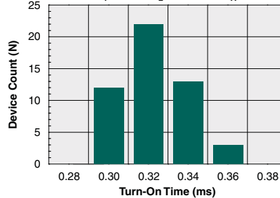
Typical Turn-On Time (N=50, I F =2mA, I L =100mA, T A =25°C)
