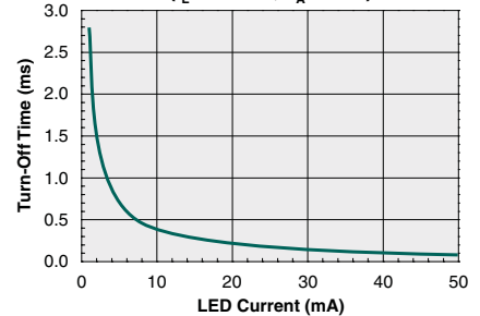
Typical Turn-Off Time vs. LED Forward Current (I L =100mA, T A =25°C)
