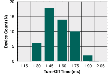
Typical Turn-Off Time (N=50, I F =2mA, I L =100mA, T A =25°C)
