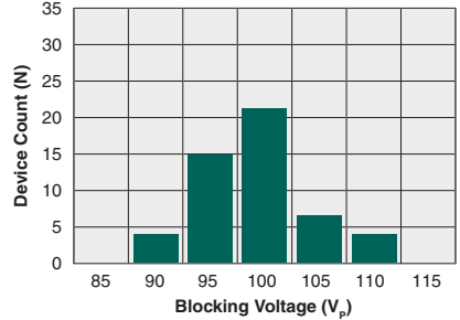
Typical Blocking Voltage Distribution (N=50, I F =1mA, T A =25°C)
