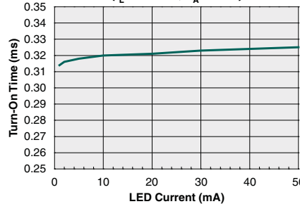
Typical Turn-On Time vs. LED Forward Current (I L =100mA, T A =25°C)
