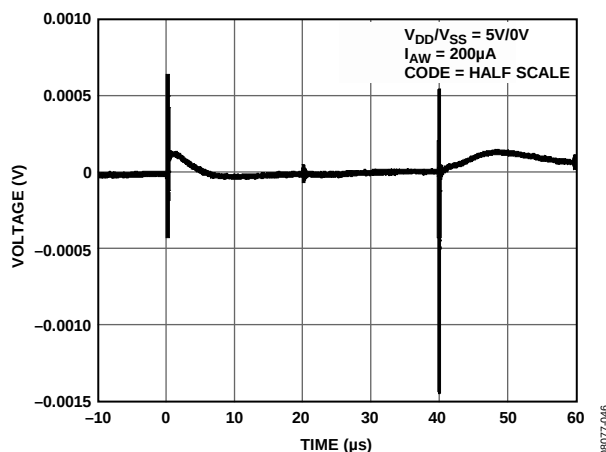
Figure 35. Digital Feedthrough
