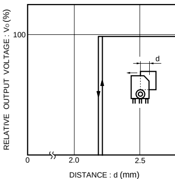
Fig.6 Relative output voltage vs. distance characteristics
