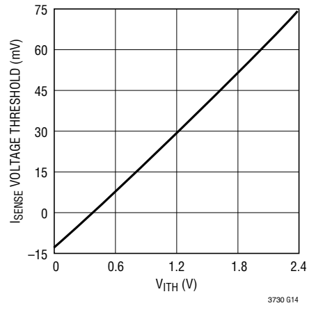
Peak Current Threshold vs V ITH
