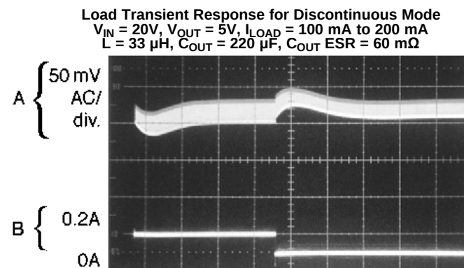
Figure 17. Horizontal Time Base: 2 \mu\text{s}/\text{div} .
