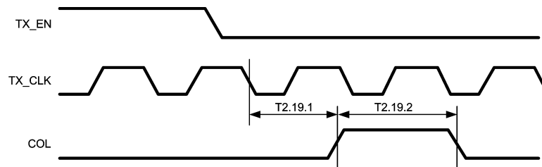
Figure 3-19. 10 Mb/s Heartbeat Timing
