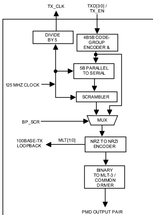
Figure 2-6. 100BASE-TX Transmit Block Diagram
