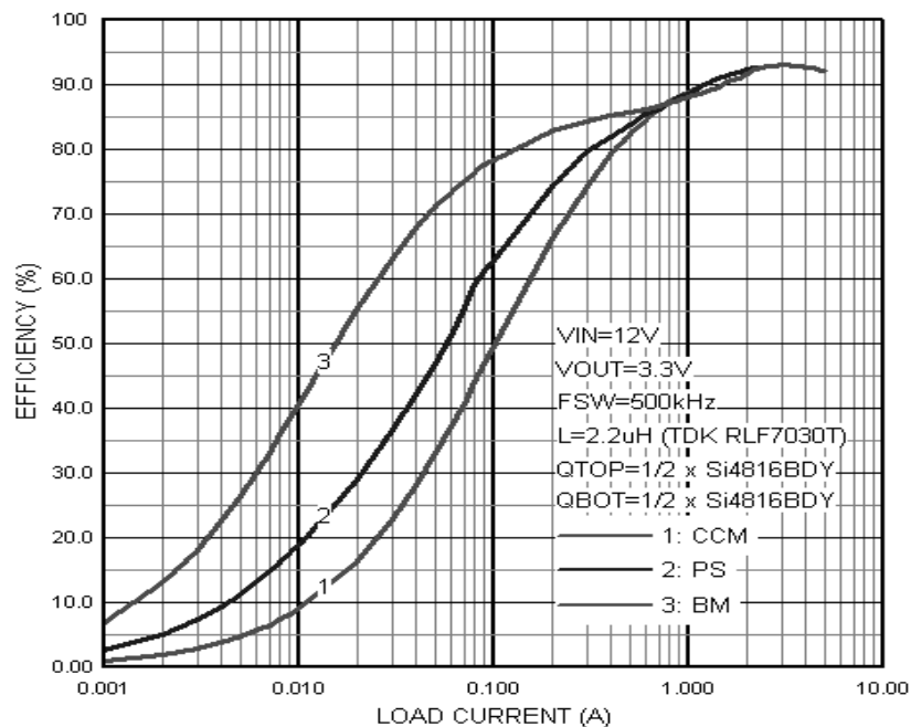
Figure 3. Efficiency vs load current For Vout1
