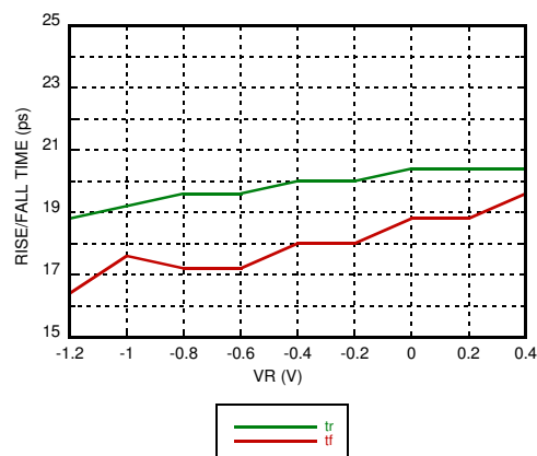
Rise / Fall Time vs. VR [2]
