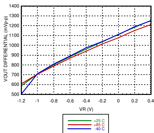
Output Differential vs. VR [2]
