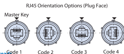
RJ45 Orientation Options (Plug Face)
