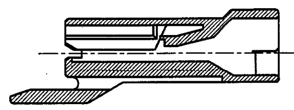
断面 "A" - "A" SECT.
