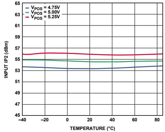
Figure 13. Input IP2 vs. Temperature
