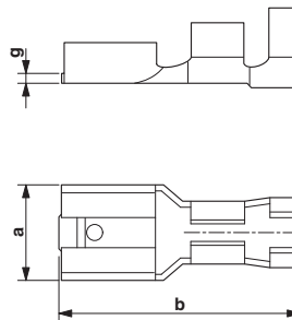
Dimensioned drawing
