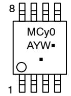
Micro8 MC34164DM CASE 846A
