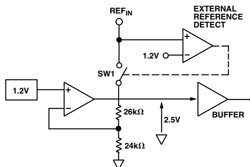
Figure 9. On-Chip Reference
