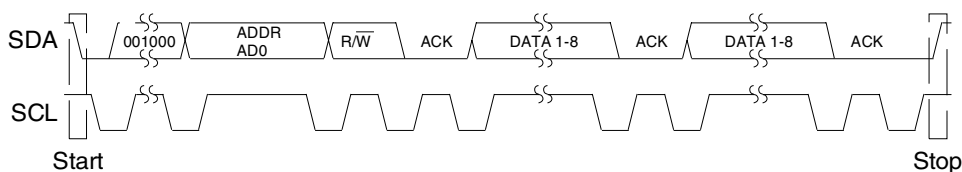
Figure 7. Control Port Timing, I²C mode
