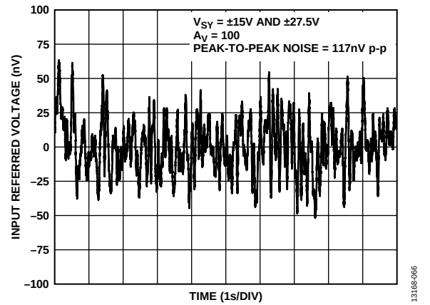
Figure 64. 0.1 Hz to 10 Hz Noise
