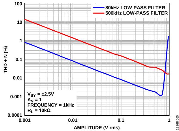
Figure 48. THD + N vs. Amplitude, V_{SY} = \pm 2.5 V
