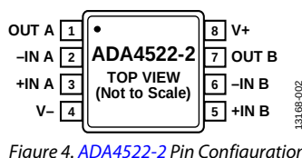
Figure 4. ADA4522-2 Pin Configuration
