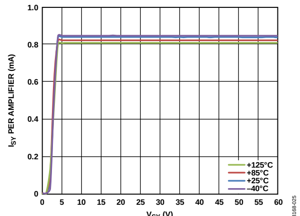
Figure 22. Supply Current ( I_{SY} ) per Amplifier vs. Supply Voltage ( V_{SY} )
