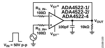
Figure 75. Circuit Diagram for Large Signal Transient Response
