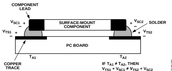
Figure 85. Mismatch in Seebeck Voltages Causes Seebeck Voltage Error
