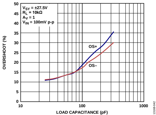
Figure 44. Small Signal Overshoot vs. Load Capacitance, V_{SV} = \pm 27.5 V
