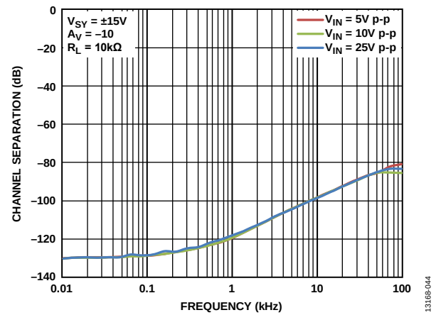
Figure 46. Channel Separation vs. Frequency, V_{SV} = \pm 15 V
