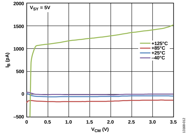
Figure 15. Input Bias Current ( I_B ) vs. Common-Mode Voltage ( V_{CM} ), V_{SY} = 5\text{ V}
