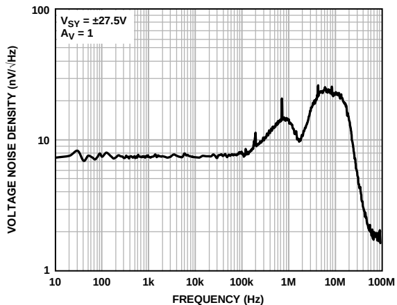
Figure 62. Voltage Noise Density vs. Frequency, V_{SV} = \pm 27.5V
