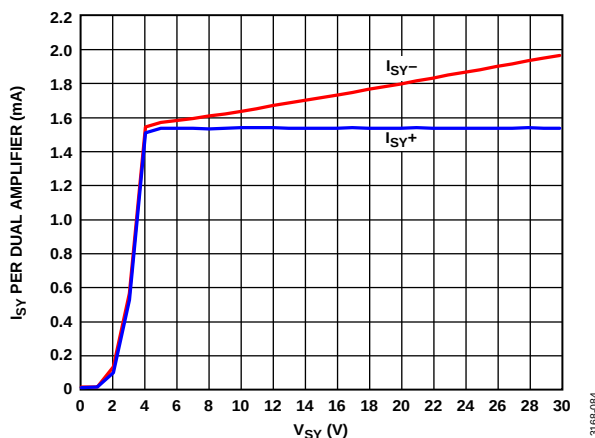
Figure 88. Supply Current ( I_{SY} ) per Dual Amplifier vs. Supply Voltage ( V_{SV} ) ( ADA4522-1/ADA4522-2/ADA4522-4 as a Comparator)
