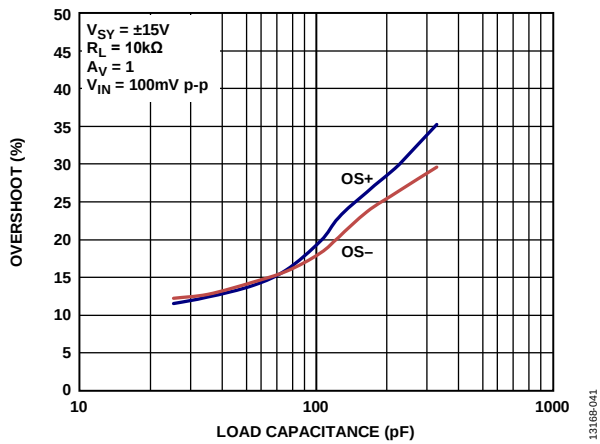
Figure 43. Small Signal Overshoot vs. Load Capacitance, V_{SV} = \pm 15 V
