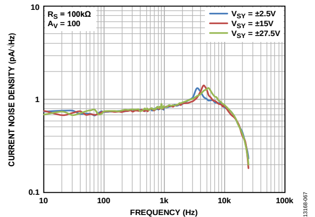
Figure 65. Current Noise Density vs. Frequency
