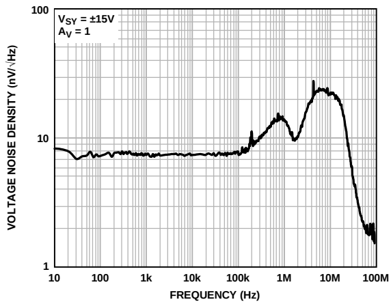
Figure 61. Voltage Noise Density vs. Frequency, V_{SV} = \pm 15V
