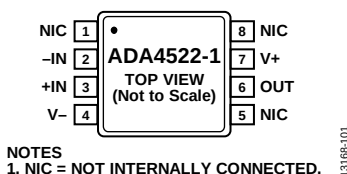
Figure 3. ADA4522-1 Pin Configuration
