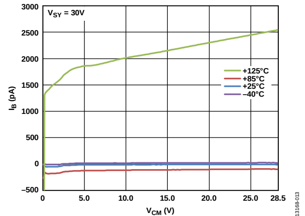
Figure 16. Input Bias Current ( I_B ) vs. Common-Mode Voltage ( V_{CM} ), V_{SY} = 30\text{ V}
