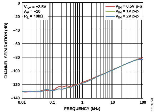
Figure 45. Channel Separation vs. Frequency, V_{SV} = \pm 2.5 V
