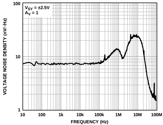
Figure 60. Voltage Noise Density vs. Frequency, V_{SV} = \pm 2.5V
