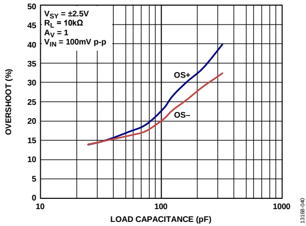
Figure 42. Small Signal Overshoot vs. Load Capacitance, V_{SV} = \pm 2.5 V
