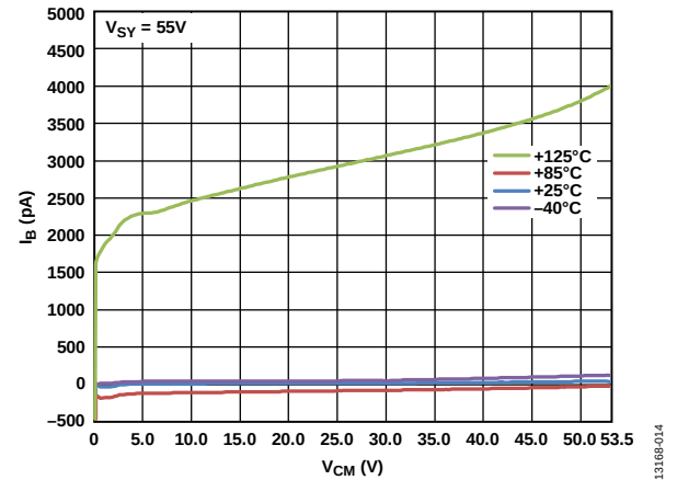
Figure 17. Input Bias Current ( I_B ) vs. Common-Mode Voltage ( V_{CM} ), V_{SY} = 55\text{ V}
