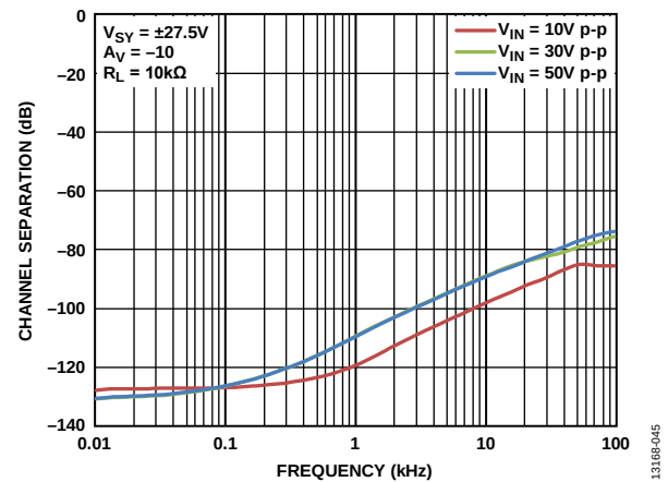
Figure 47. Channel Separation vs. Frequency, V_{SV} = \pm 27.5 V
