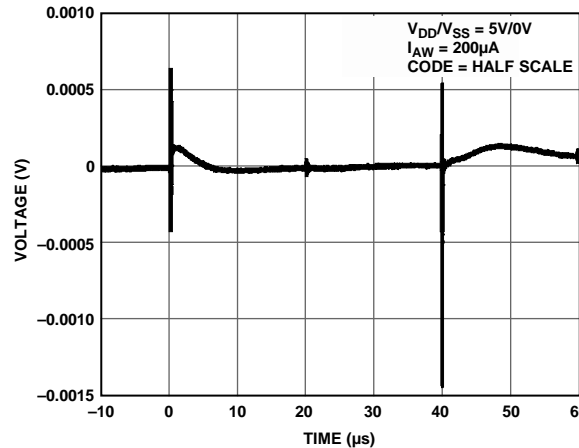
Figure 35. Digital Feedthrough
