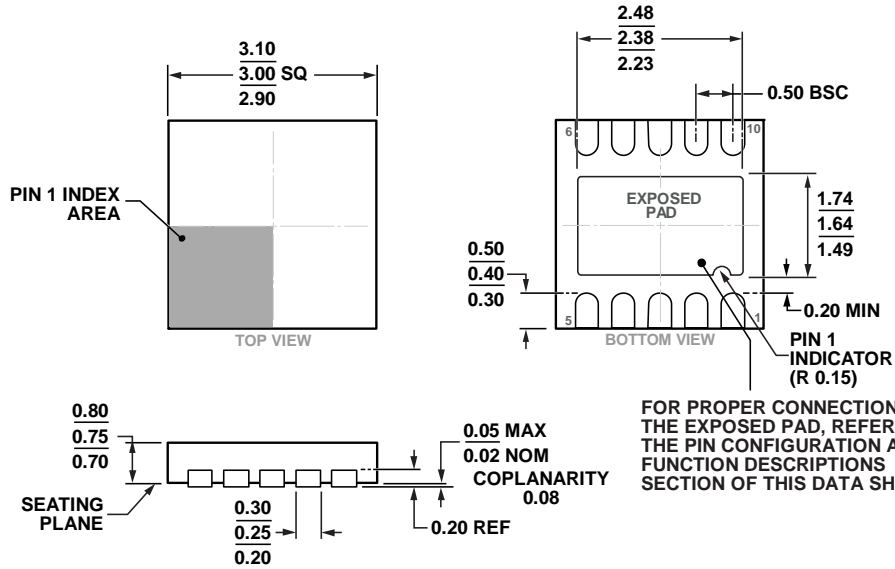
Figure 49. 10-Lead Frame Chip Scale Package [LFCSF_WD] 3 mm × 3 mm Body, Very Thin, Dual Lead (CP-10-9) Dimensions shown in millimeters
