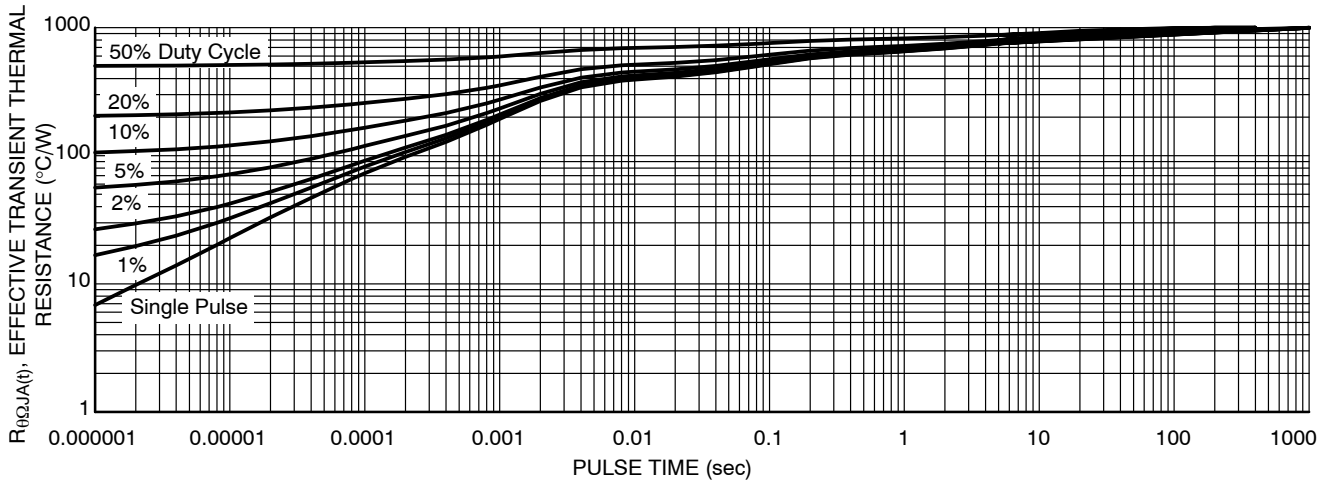
Figure 22. Thermal Response
