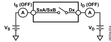
Figure 28. Off Leakage
