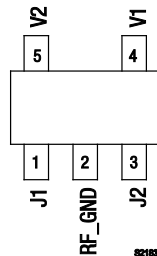
Figure 2. AA103-72/-72LF Pinout – 5-Pin SOT-5 (Top View)
