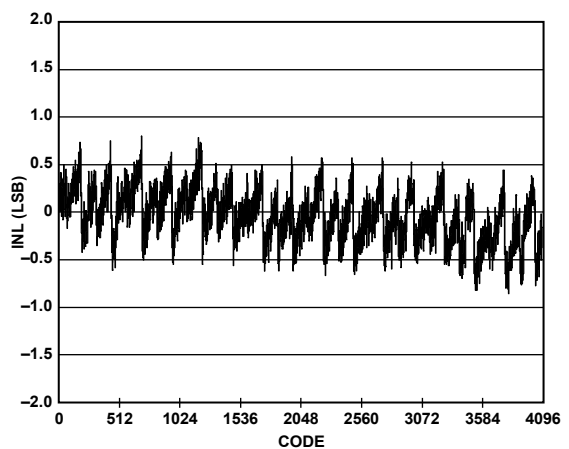
Figure 14. ADC INL
