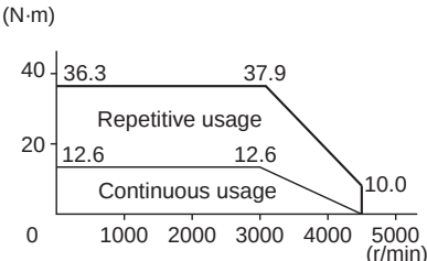
R88M-G5K030T (5 kW)
