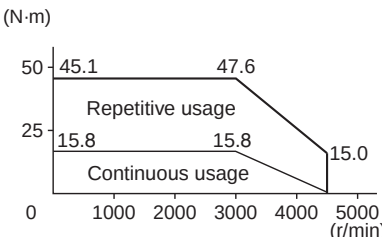
R88M-G4K030T (4 kW)
