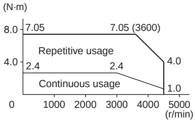
R88M-G75030H/T (750 W)
