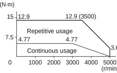
R88M-G1K530T (1.5 kW)
