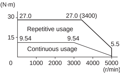
R88M-G3K030T (3 kW)
