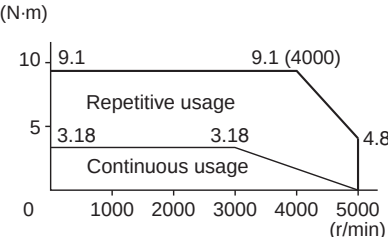
R88M-G1K030T (1 kW)
