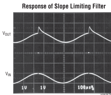
Figure 2. Lowpass Slope Limiting Filter with 0 TC
