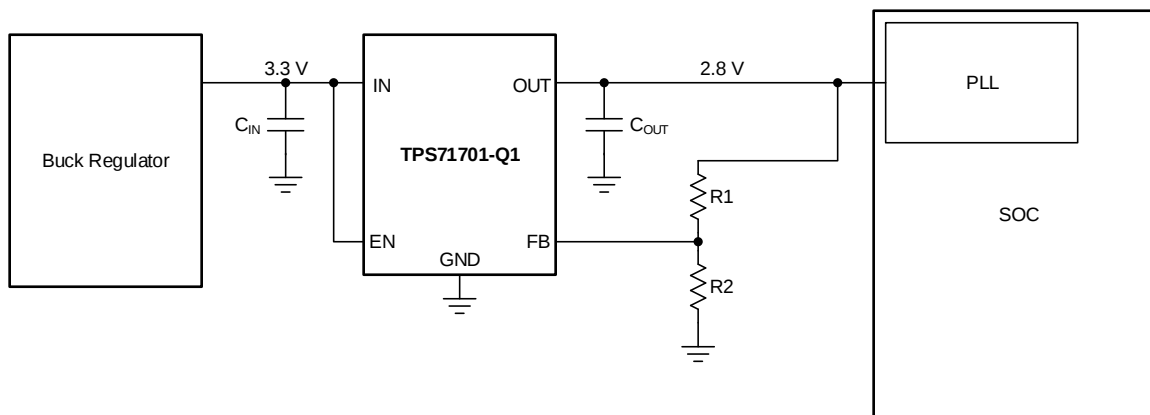
Figure 35. Typical Application Circuit: PLL on an SOC
