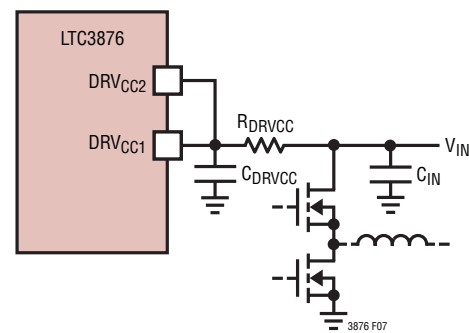
Figure 7. Setup for V IN ≤ 5.3V
