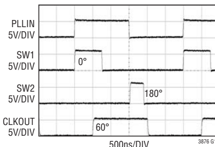
Phase Relationship: PHASMD = Ground (Forced Continuous Mode)
