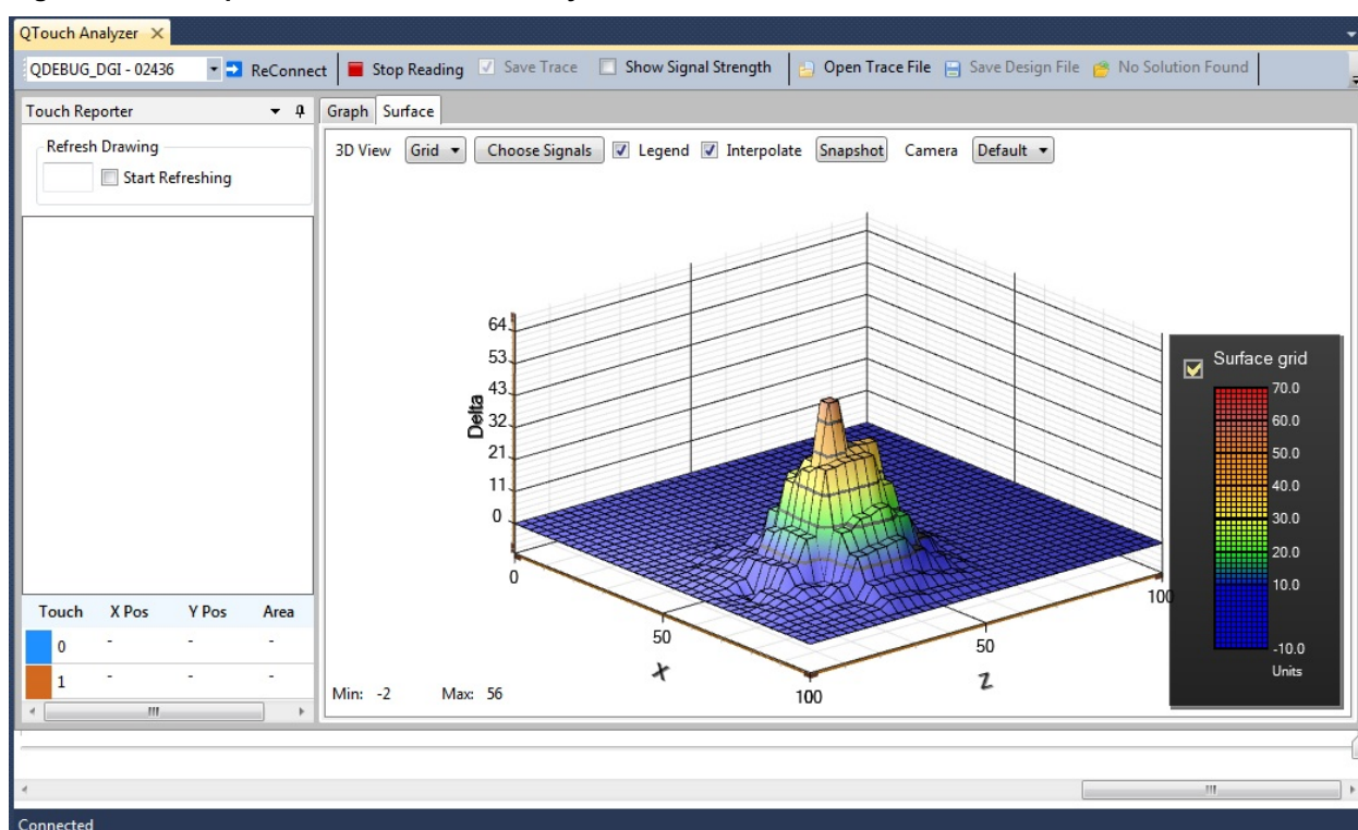
Figure 2-1. QT6 Xplained Pro in QTouch Analyzer
