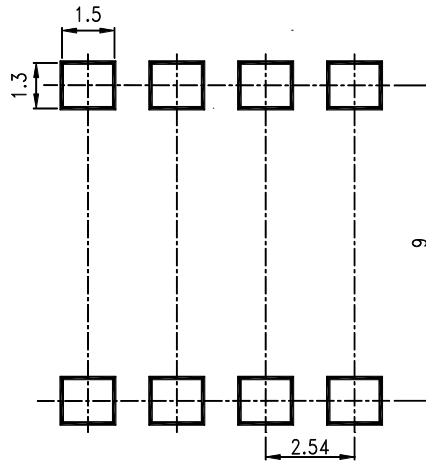
7.2 8 PIN
