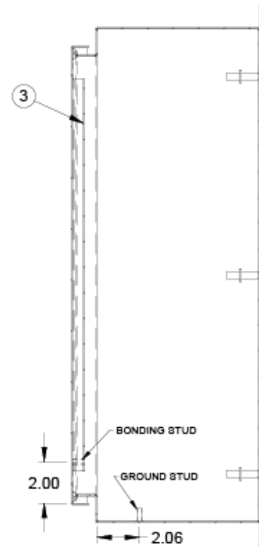
SECTION X-X
