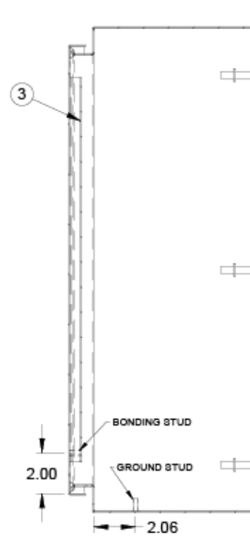
SECTION X-X
