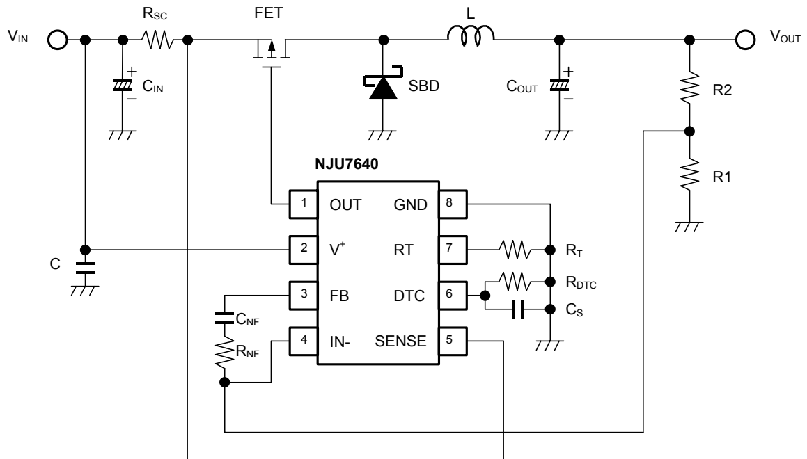
Step-Down Converter
