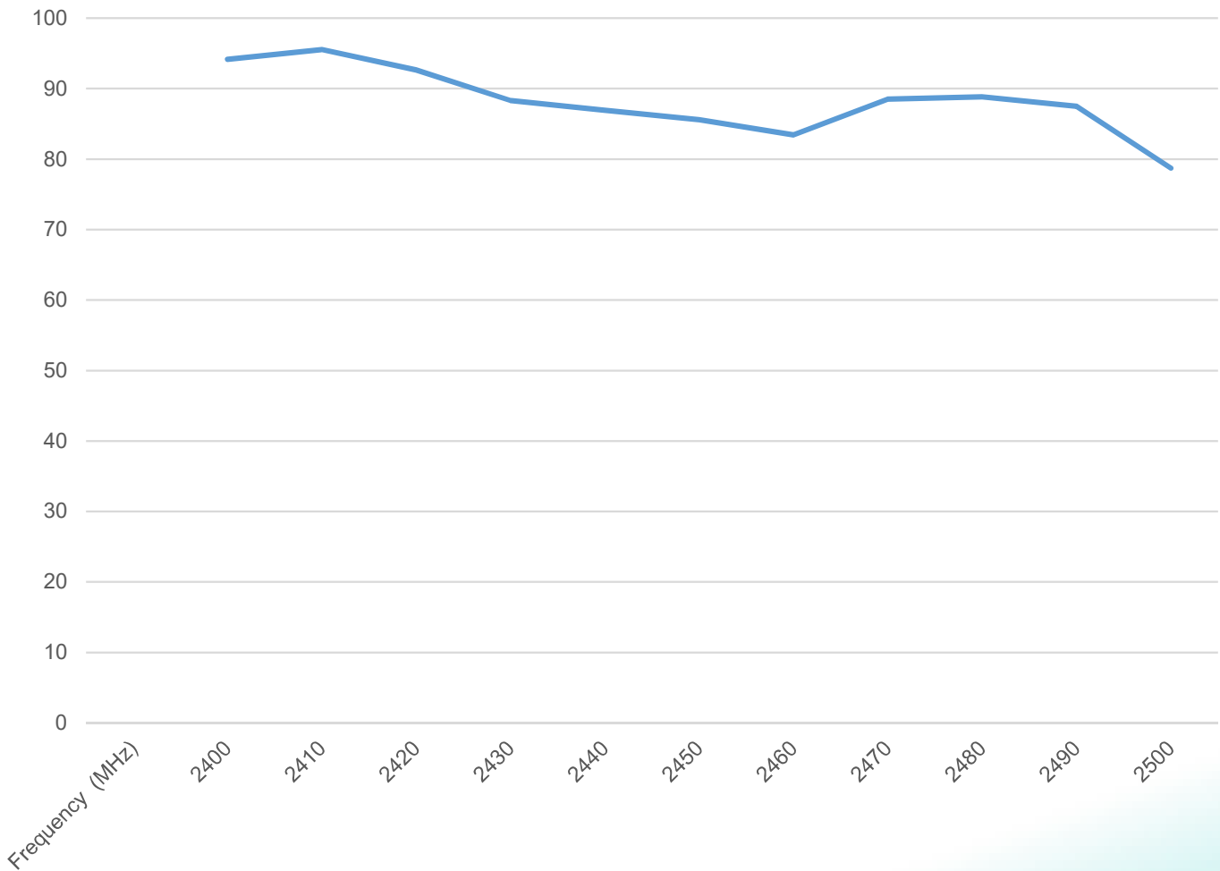
ICEFIN24NMOHF Efficiency (%)
