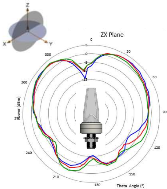
Elevation Plane
