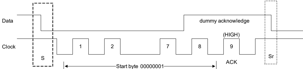
Figure 124. START Byte Transfer
