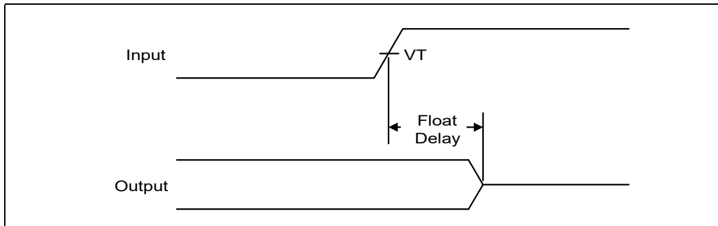
Figure 85. Pulse Width
