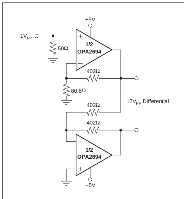
Figure 8. Single-to-Differential Conversion
