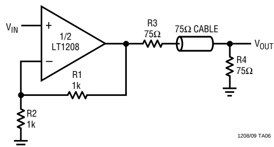
Cable Driving
