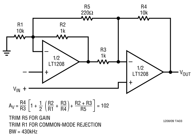
Instrumentation Amplifier
