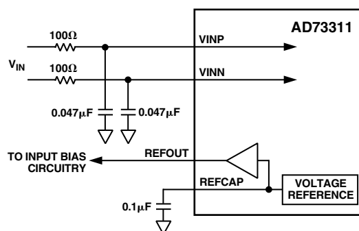
The AD73311's on-chip 38 dB preamplifier can be enabled when there is not enough gain in the input circuit; the preamplifier is configured by bits IGS0–2 of CRD. The total gain must be configured to ensure that a full-scale input signal produces a signal level at the input to the sigma-delta modulator of the ADC that does not exceed the maximum input range.
