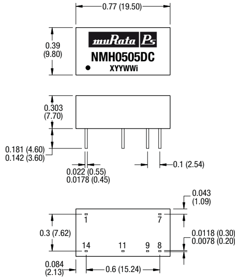
DIP package
