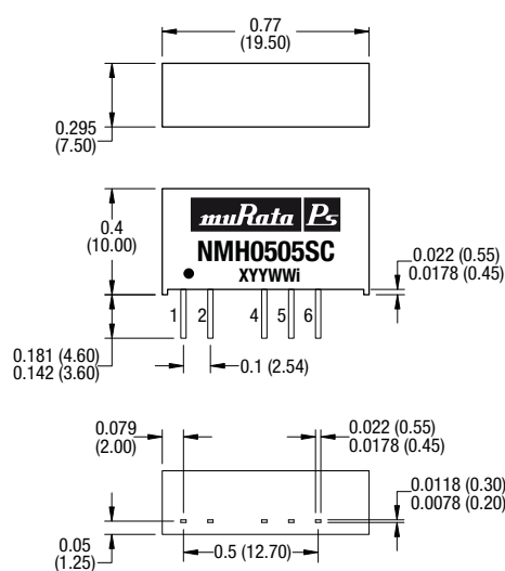
SIP package
