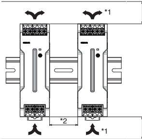
*1. Convection of air *2. 20 mm min.
