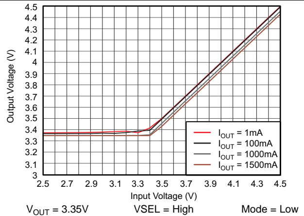
Figure 38. TPS61281 DC Output Voltage vs Input Voltage
