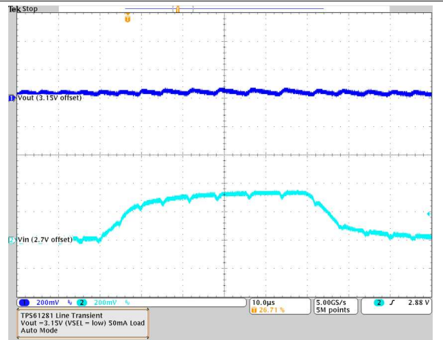
Figure 62. TPS61282 Line Transient
