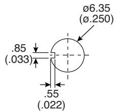
Without locking ring
