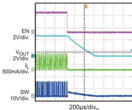
Shutdown Through EN I_{OUT} = 0.3A
